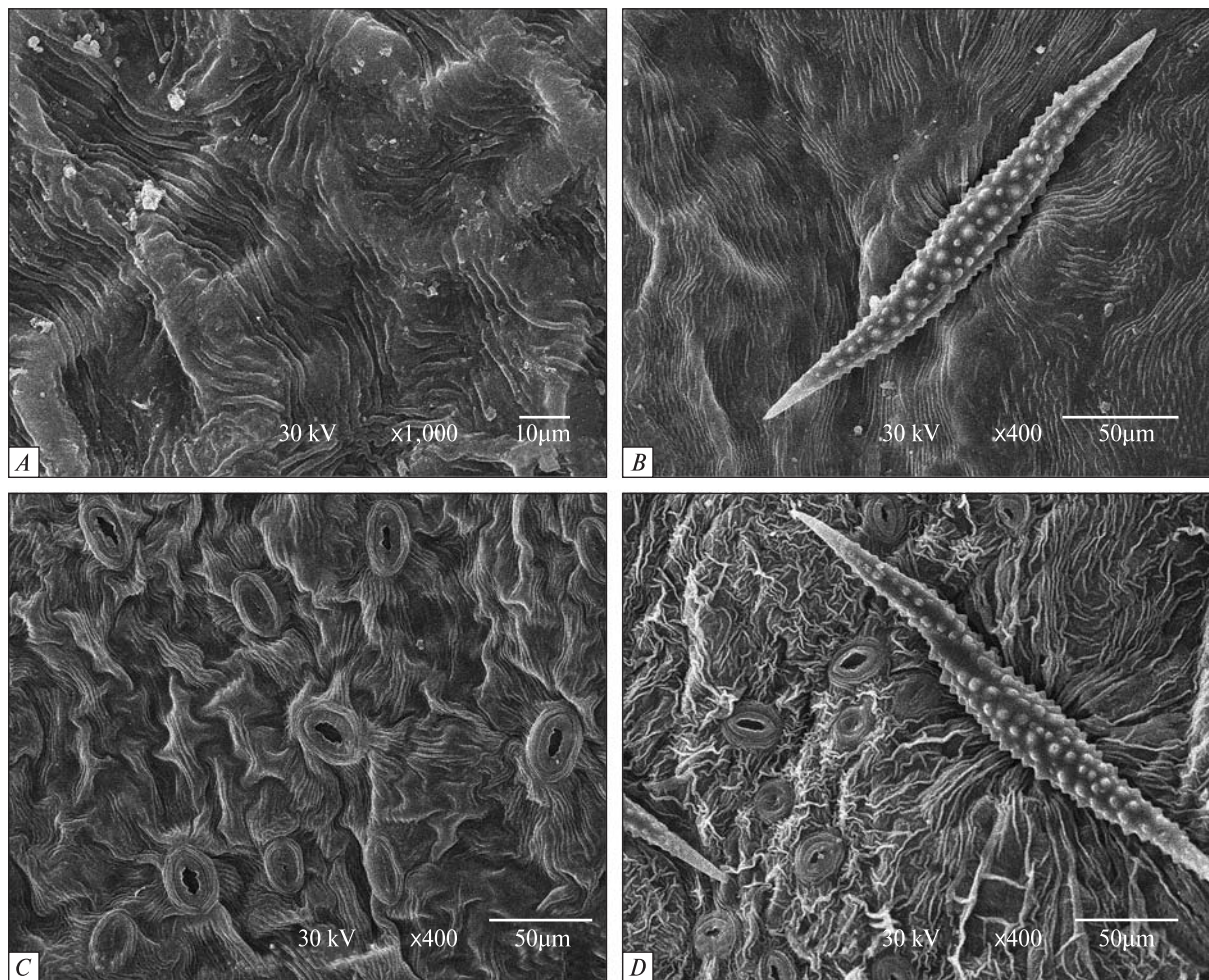
Рис. 2. Структура верхней (A, B) и нижней (C, D) поверхности листьев Cornus officinalis и Cynoxylon japonica Fig. 2. The structure of the upper (A, B) and lower (C, D) surface of Cornus officinalis and Cynoxylon japonica leaves
